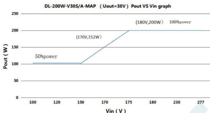
DL-200W-V38S/A-MAP(38Vdc,Rated output current and output power corresponding to different Input voltages)
