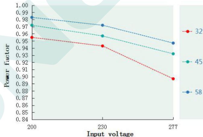
Power factor VS Input voltage(DL-200H-V58P/A-MAS)
