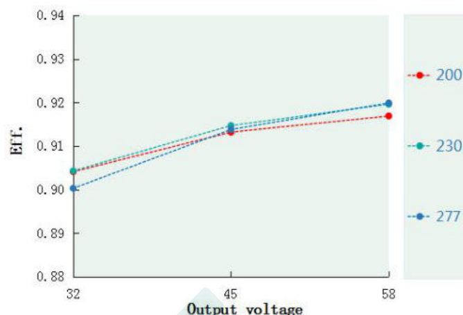
Eff. VS Output voltage(DL-200H-V58P/A-MAS)
