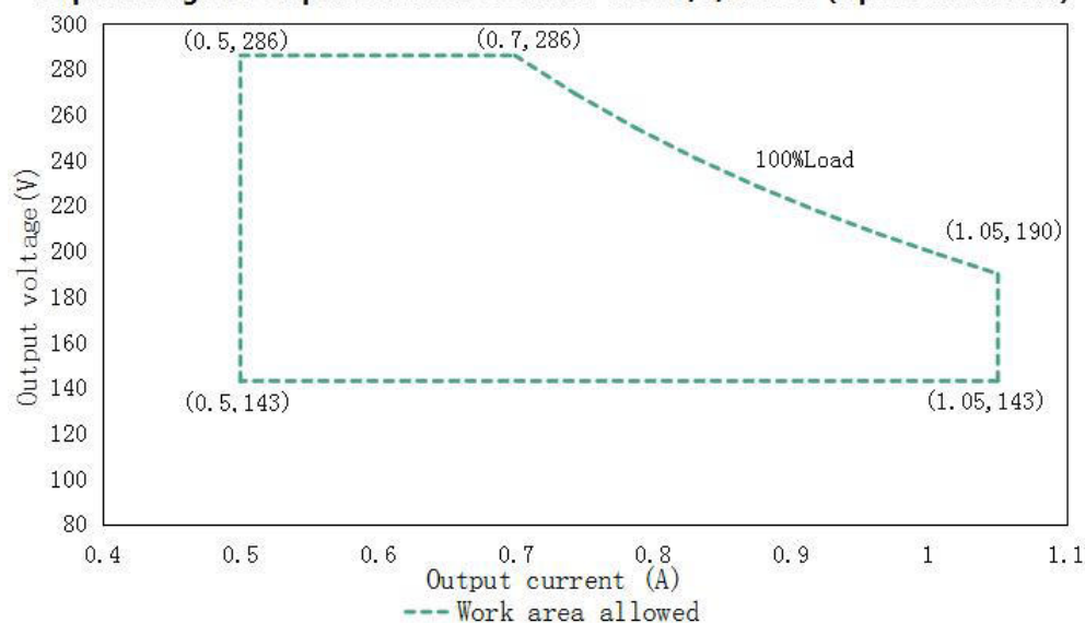
Output voltage VS output current of DL-200W-V286A/P/X-MXG (input: 120-277Vac)
