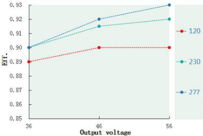
Eff. VS Output voltage(DL-240WK-V56A/P-MXG)
