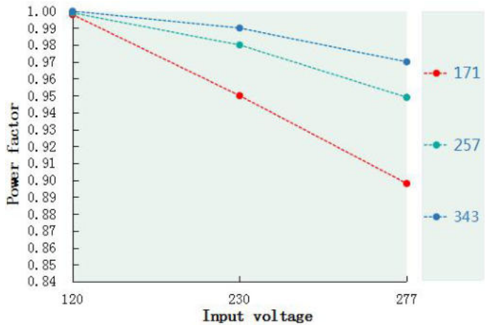
Power factor VS Input voltage(DL-240WK-V343A/P-MXG)
