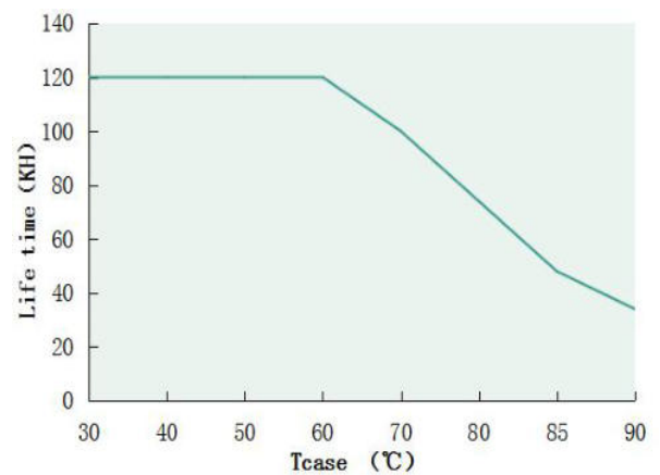
Tcase VS Lifetime
