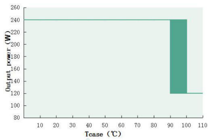
Output power VS Tcase (DL-240H-P/A-MAS)
