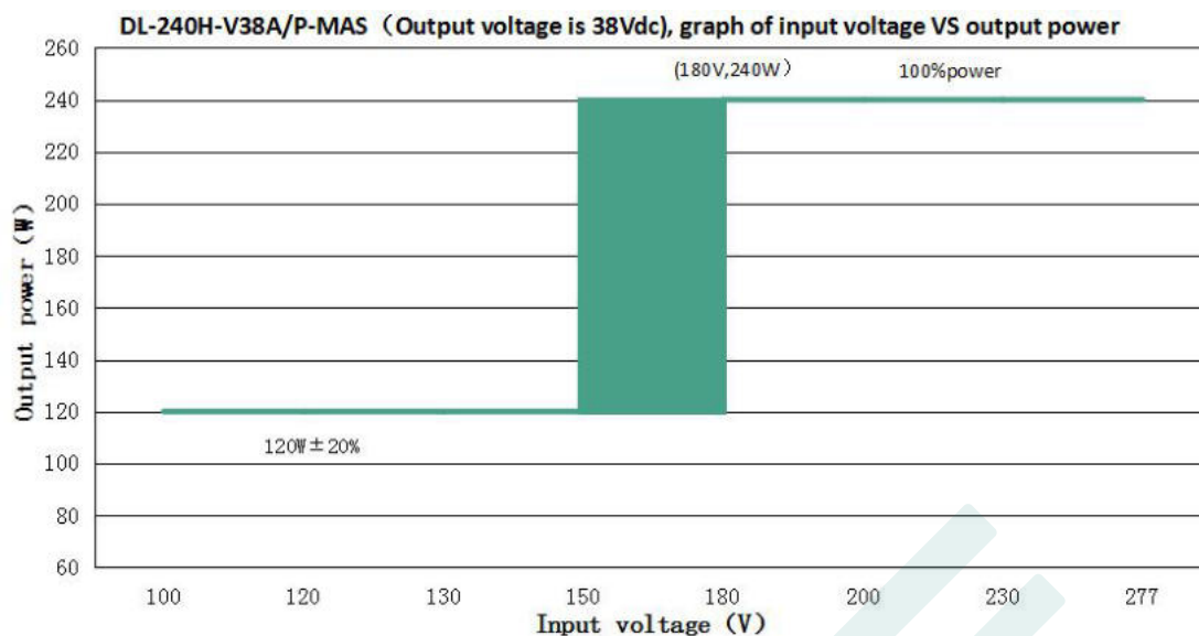
DL-240H-V38A/P-MAS(When the output voltage is 38Vdc, the rated output current value and output power corresponding to different input voltage)
