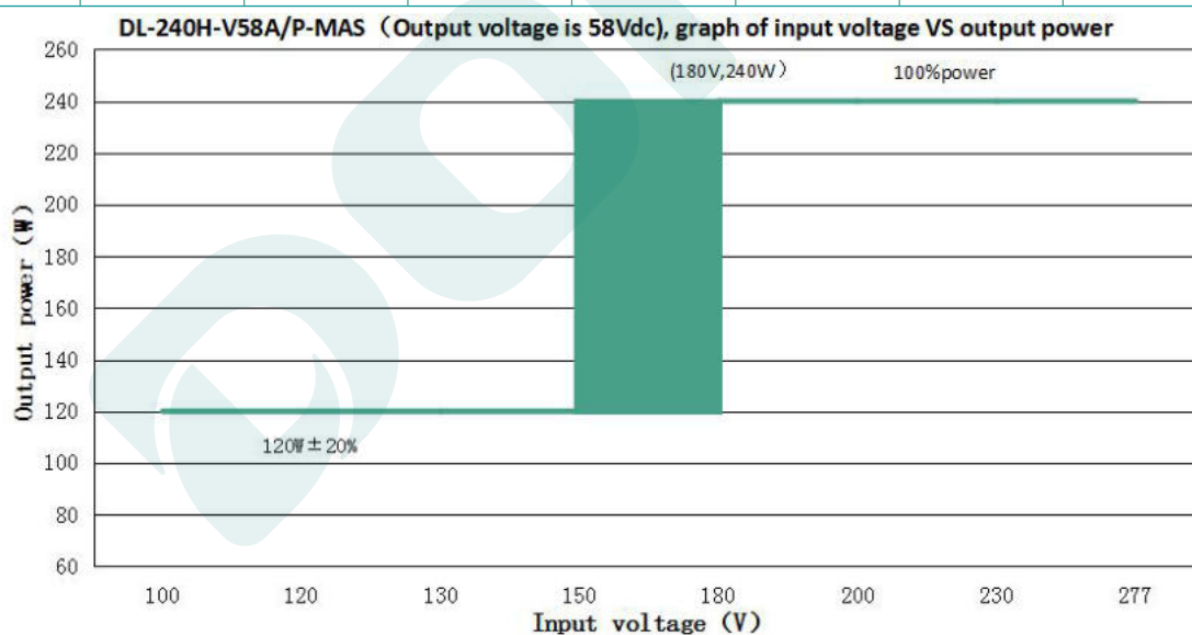
DL-240H-V58A/P-MAS (When the output voltage is 58Vdc, the rated output current value and output power corresponding to different input voltage)
