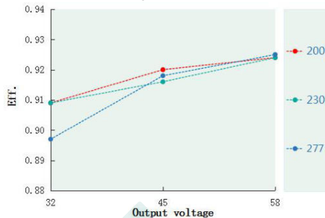
Eff. VS Output voltage(DL-240H-V58P/A-MAS)
