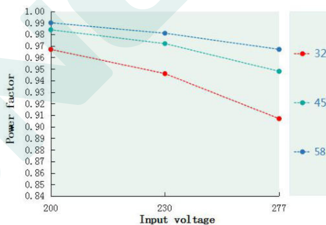
Power factor VS Input voltage(DL-240H-V58P/A-MAS)
