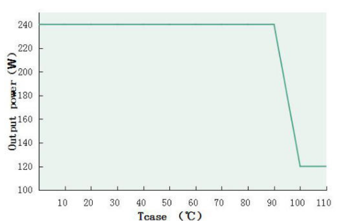
Output power VS Tcase (DL-240W-V56A/P/X-MDK)
