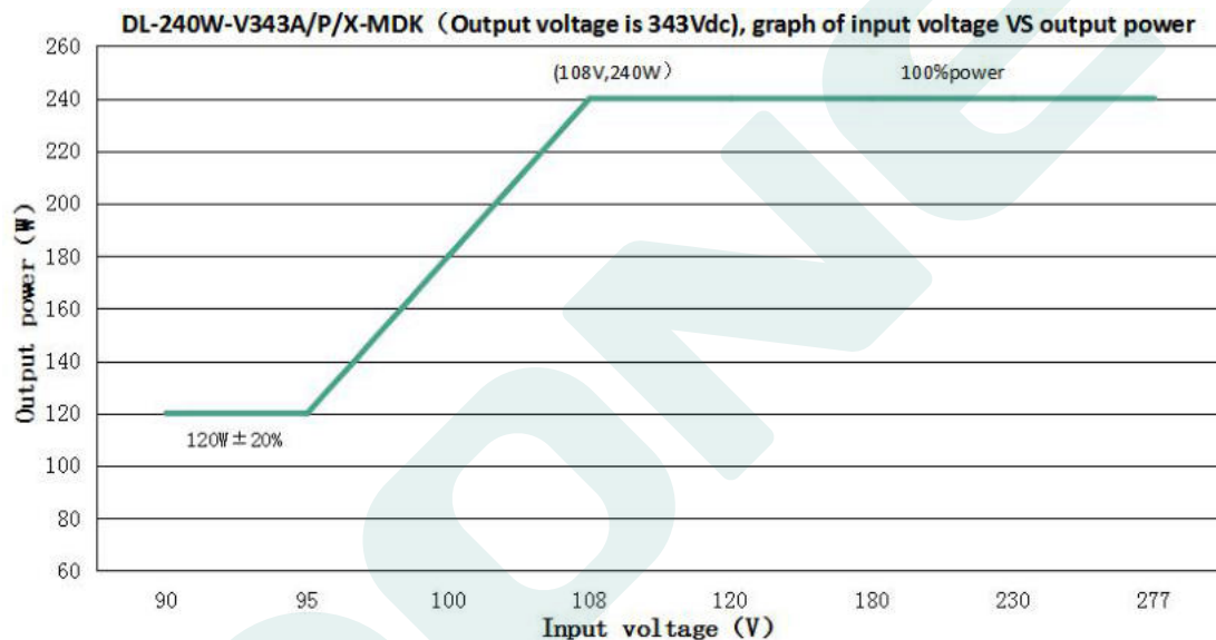
DL-240W-V343A/P/X-MDK (When the output voltage is 343Vdc, the rated output current value and output power corresponding to different input voltage)
