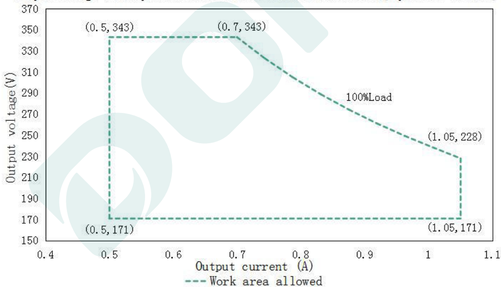
Output voltage VS output current of DL-240W-V343A/P/X-MDK (input: 120-277Vac)
