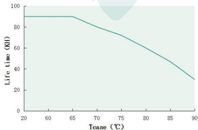
Tcase VS Lifetime(DL-400W-V260X/T-PLS)
