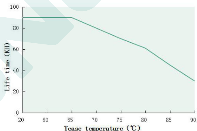
Tcase temperature VS Lifetime(DL-50H-MXC)
