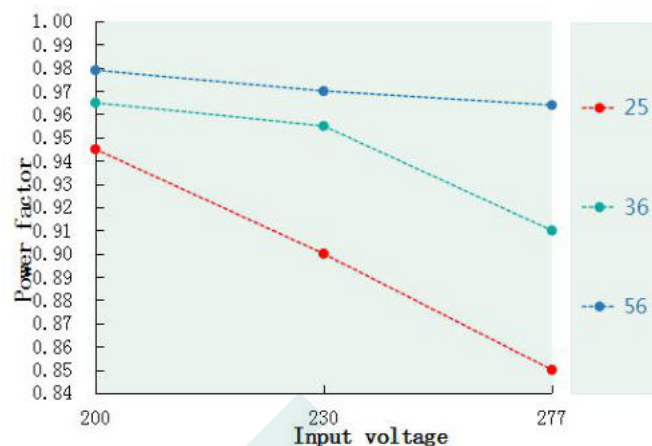
Power factor VS Input voltage((DL-50H-56A/P-MXC)
