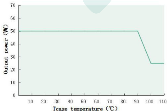
Output power VS Tcase temperature(DL-50H-MXC)
