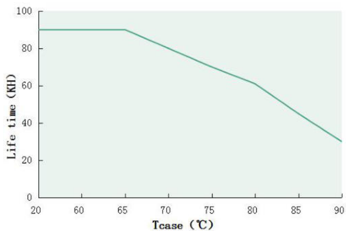
Tcase VS Lifetime(DL-50WK-A/P-MXG)
