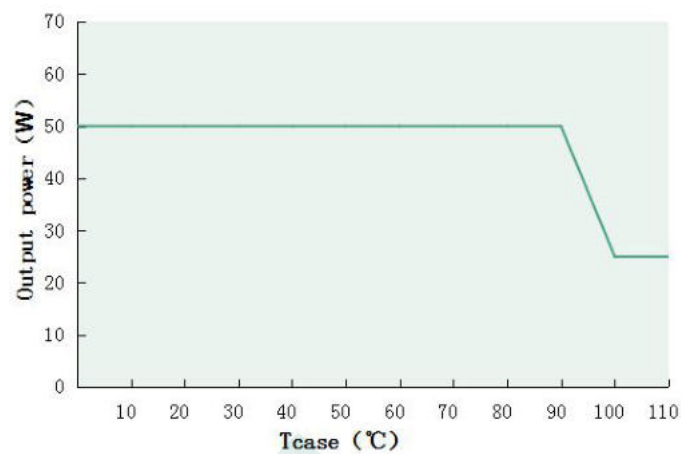
Output power VS Tcase (DL-50WK-A/P-MXG)
