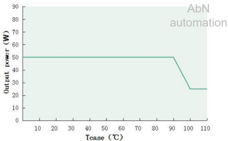
Output power VS Tcase (DL-50W-DX-MXG)
