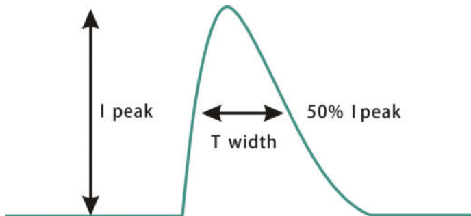
Inrush current(DL-50W-DX-MXG)
