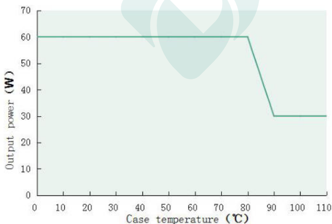
Output power VS Tcase (DL-60H-56A/P-MXC)
