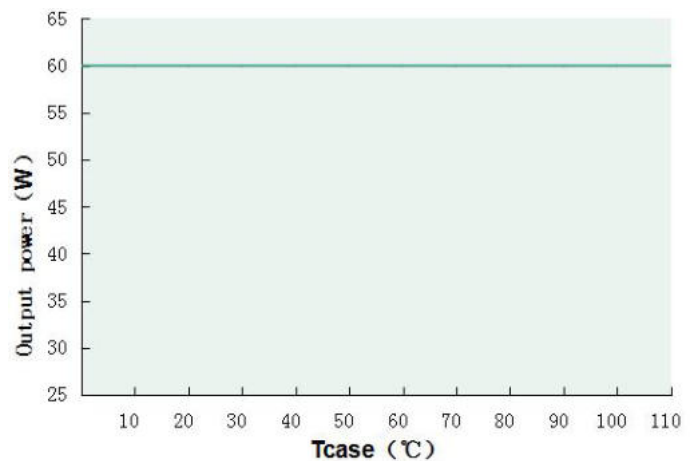
Output power VS Tcase (DL-60Z-260A/S-PXG)
