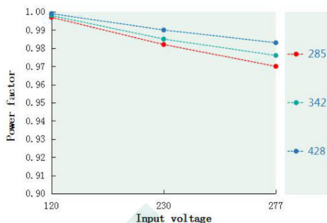
Power factor VS Input voltage(DL-720W-V428X/T-MXG)
