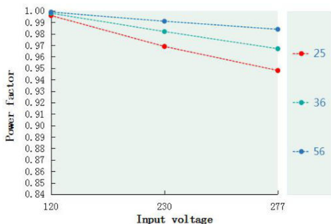
Power factor VS Input voltage(DL-720W-V56X/T-MXG)
