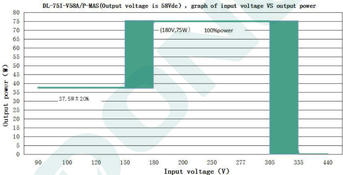
Output power versus Input voltage
