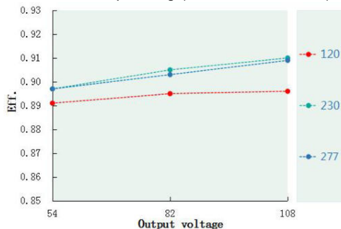
Eff. VS Output voltage(DL-75WK-V108A/P-MXG)
