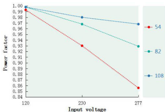
Power factor VS Input voltage(DL-75W-V108A/P/X-MDK)
