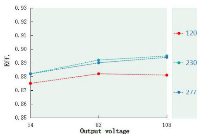
Eff. VS Output voltage(DL-75W-V108A/P/X-MDK)
