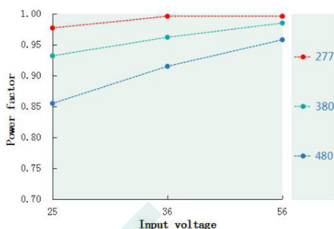
Power factor VS Input voltage(DL-800U-56X-MUG)
