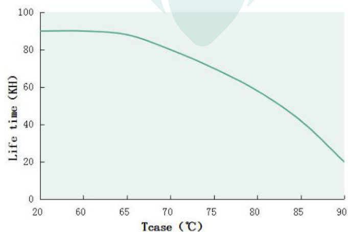
Tcase VS Lifetime(DL-800W-MUG)
