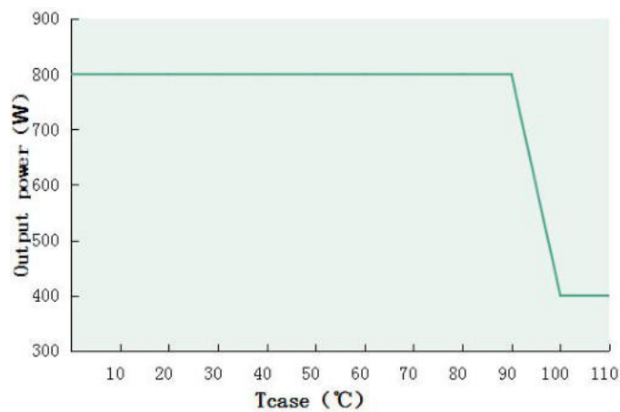
Output power VS Tcase (DL-800W-MUG)
