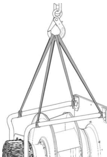
Fig. 1: Hoisting diagram for transportation of RadiPac
