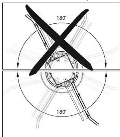
Fig. 2: Cable routing for fans installed upright.
