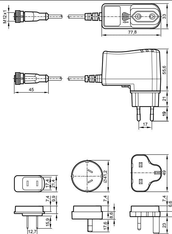
Figure shows plug-in power supply with connected EU mains adapter
