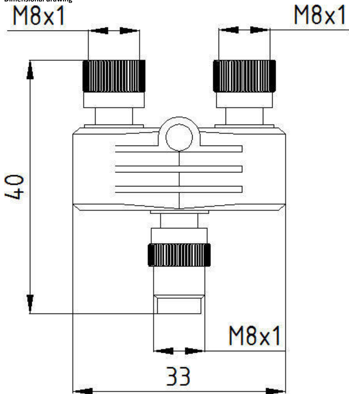
Dimensional drawing
