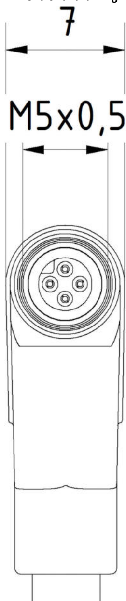
Dimensional drawing
