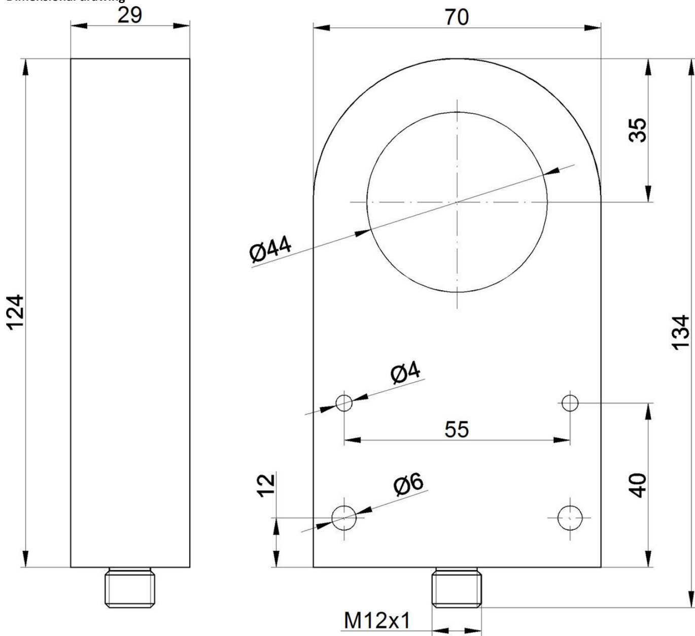
Dimensional drawing
