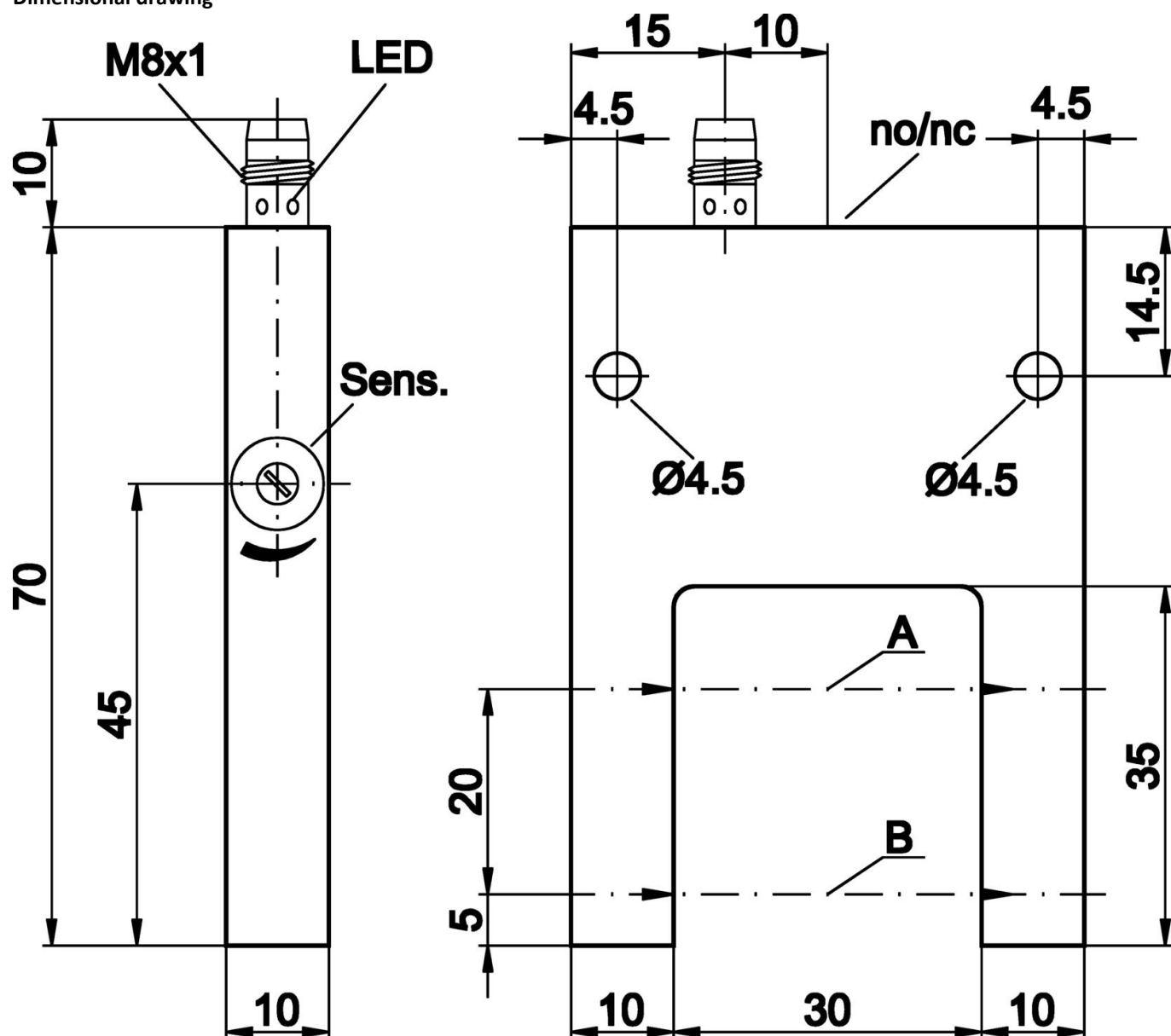
Dimensional drawing
