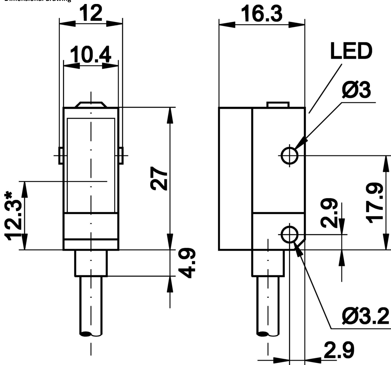
Dimensional drawing
