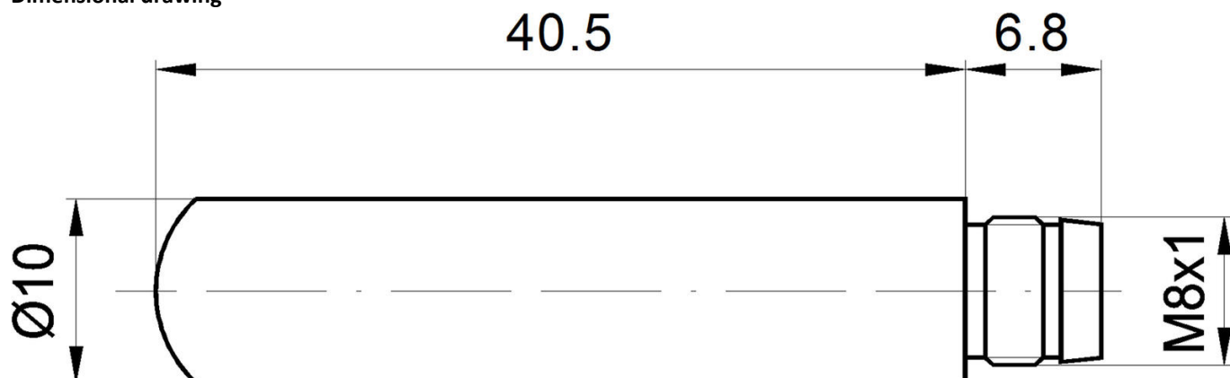
Dimensional drawing
