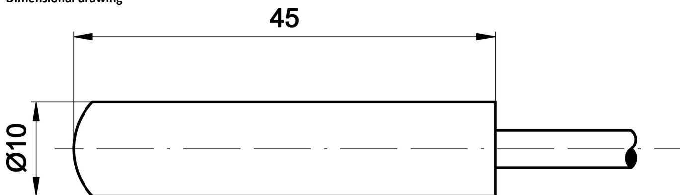
Dimensional drawing
