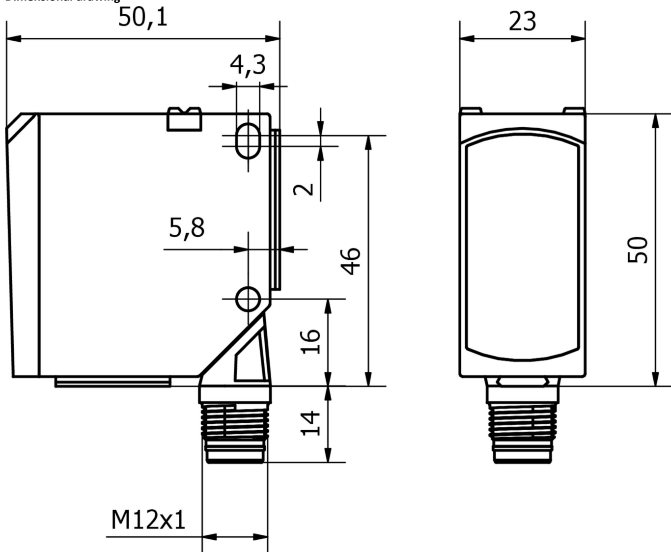
Dimensional drawing
