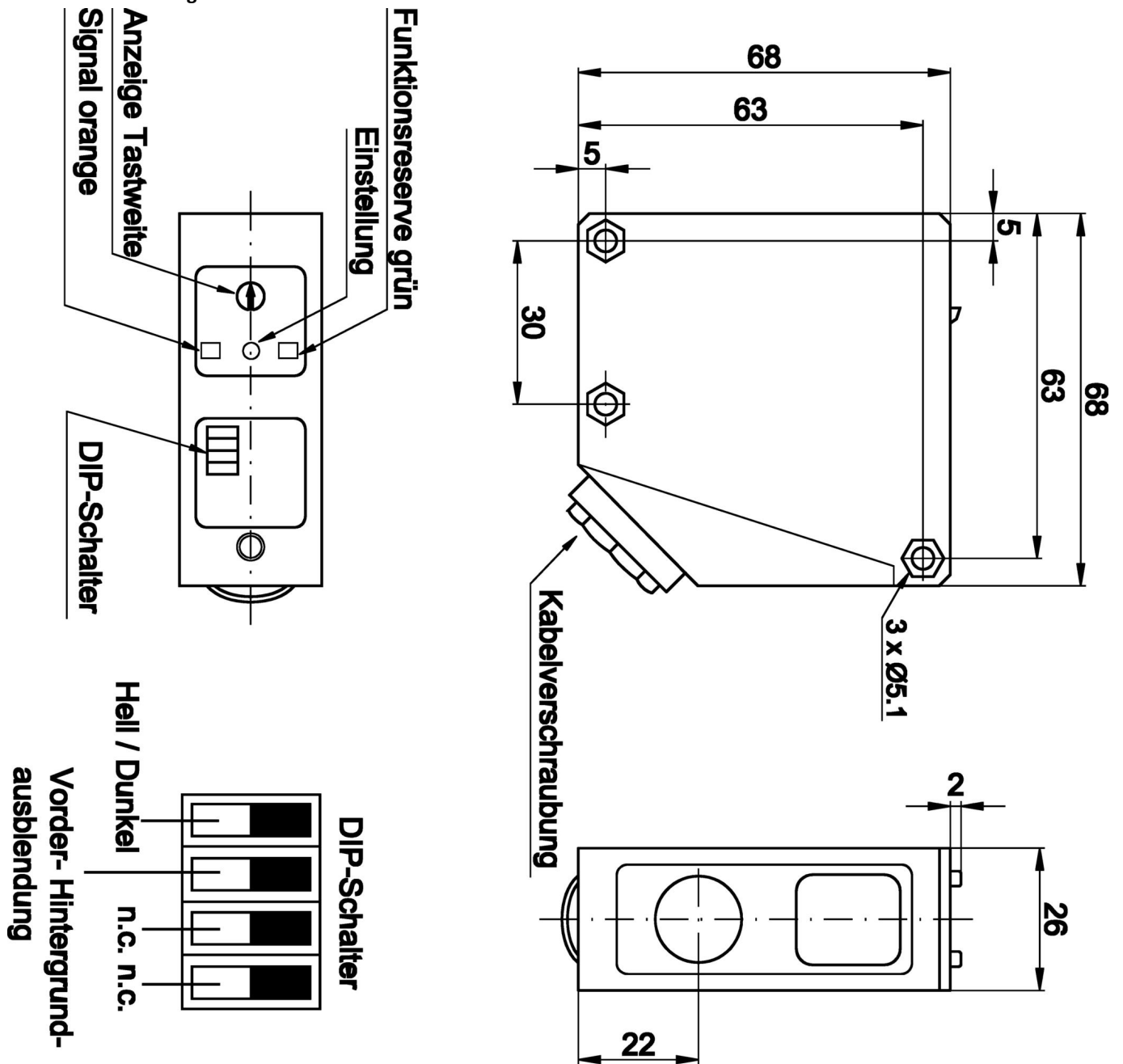
Dimensional drawing
