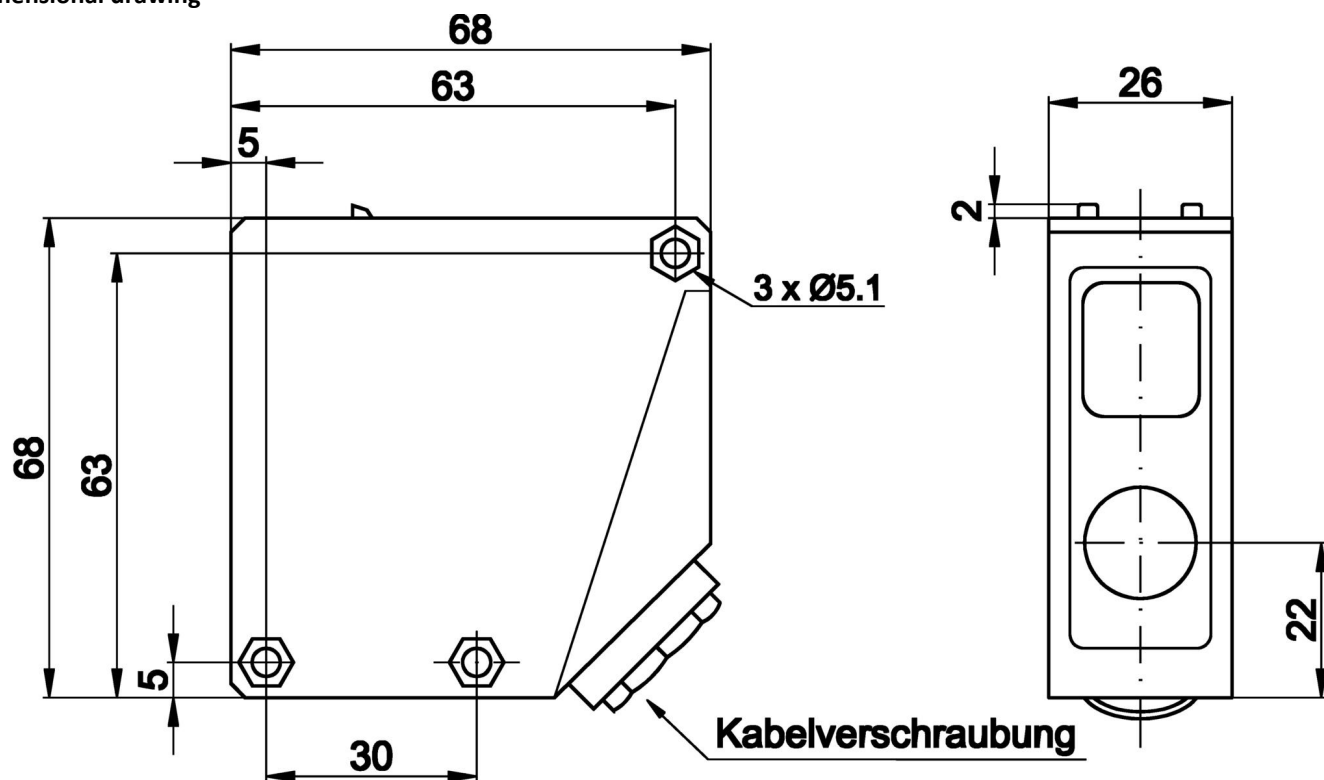
Dimensional drawing
