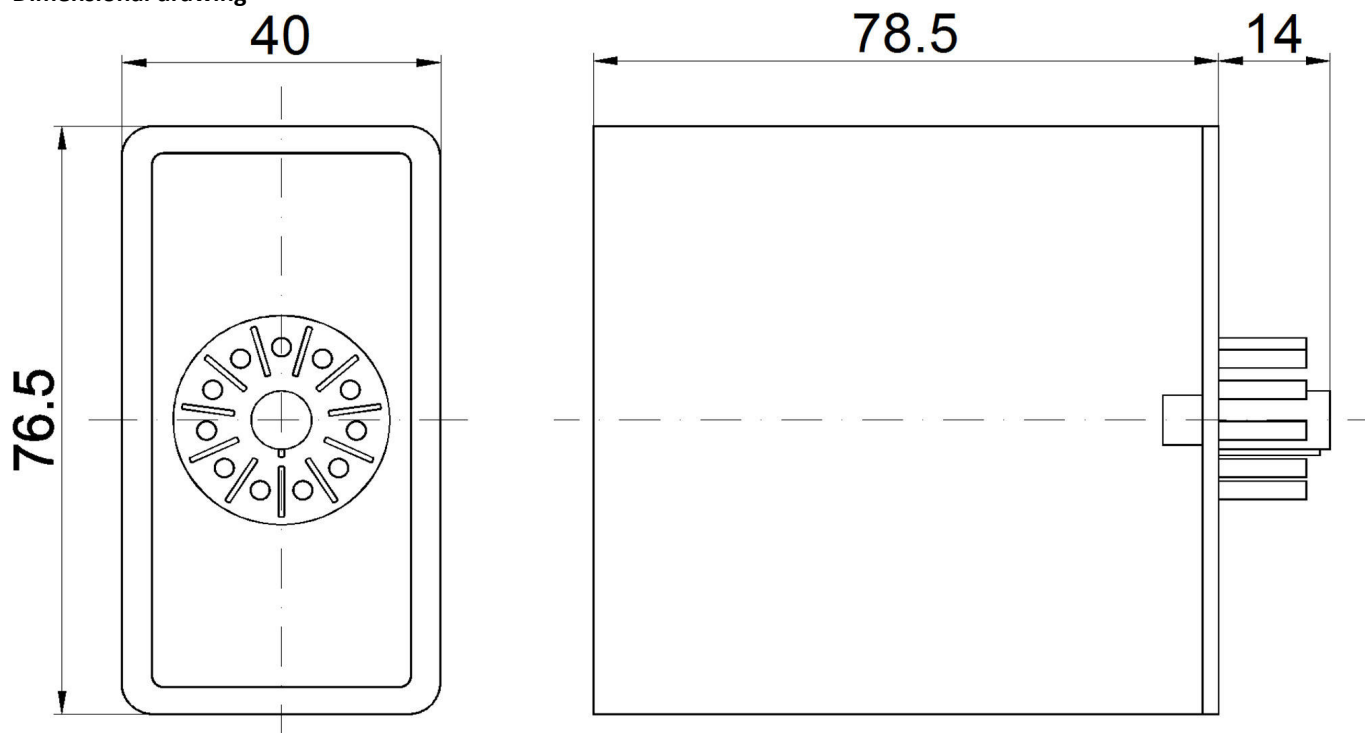
Dimensional drawing
