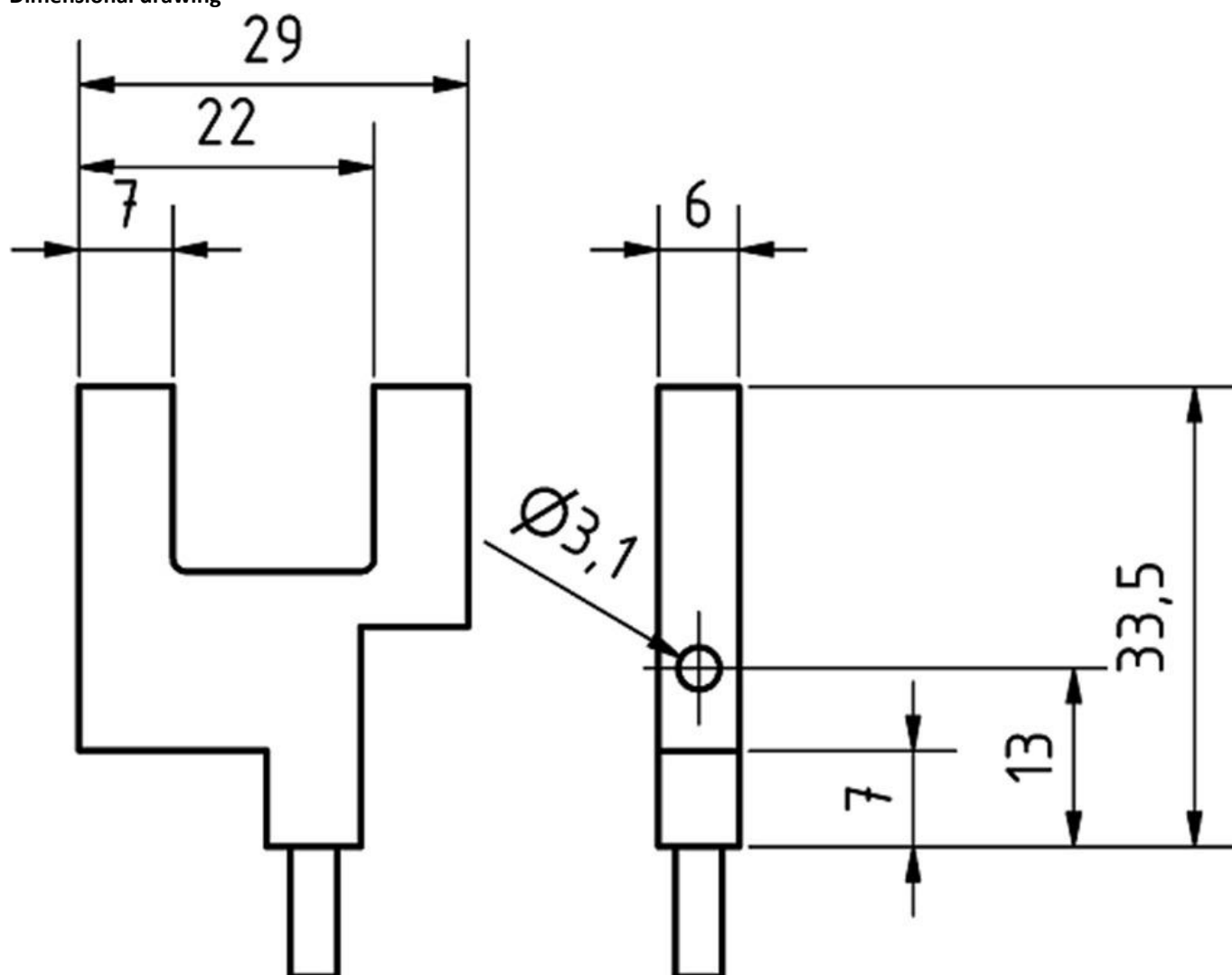
Dimensional drawing
