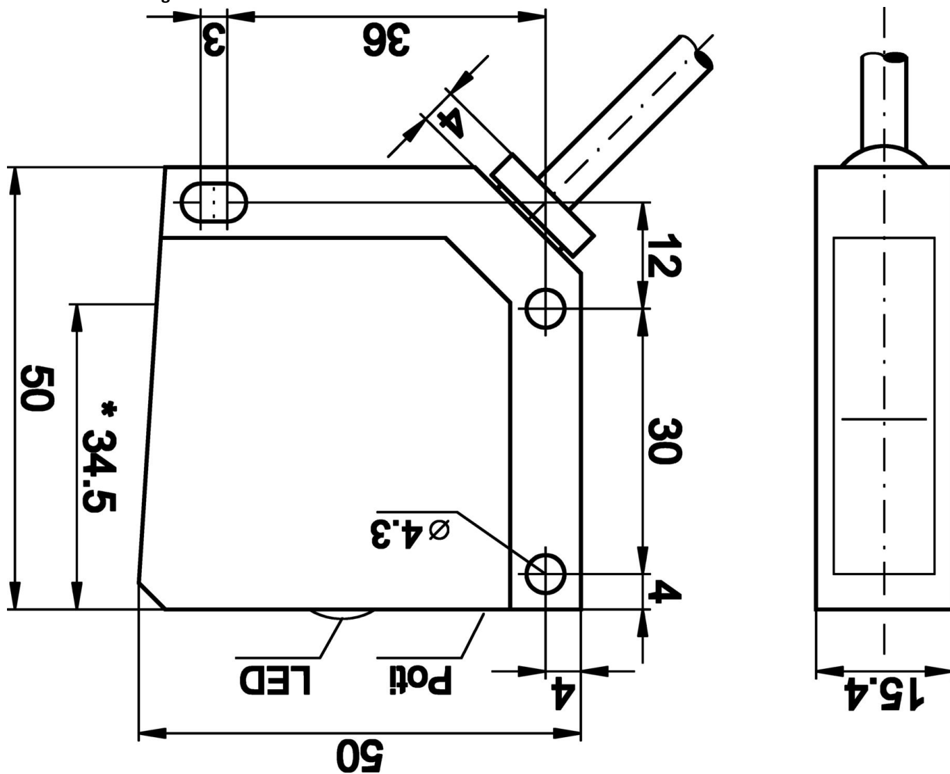
Dimensional drawing
