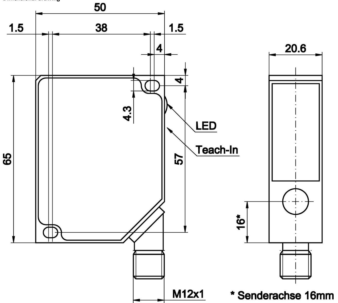
Dimensional drawing
