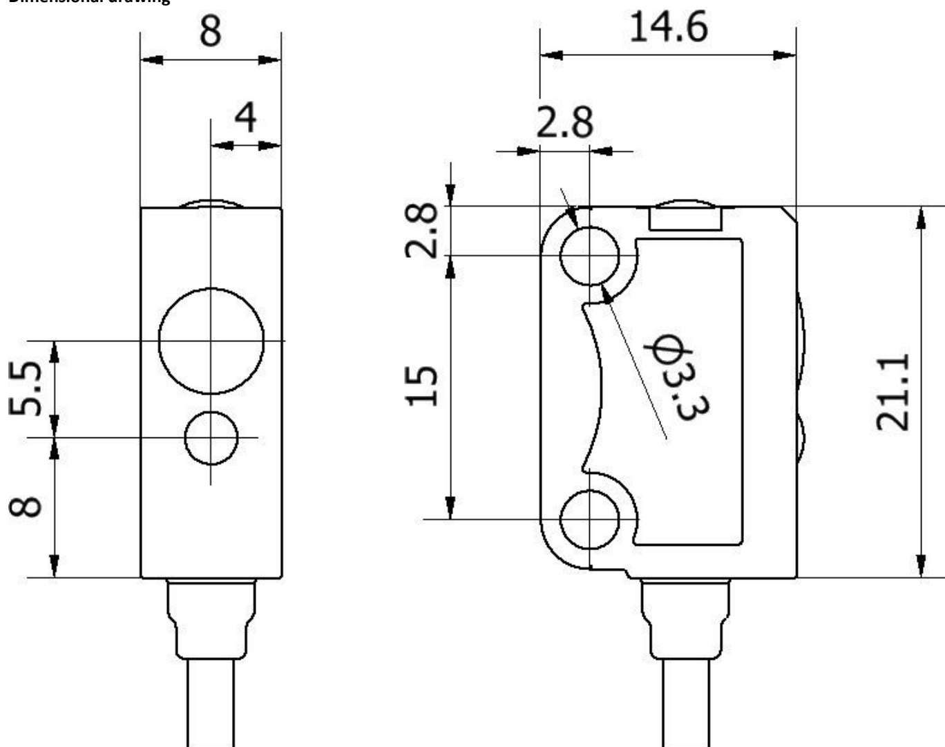
Dimensional drawing
