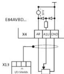
Connection of analog inputs and outputs
