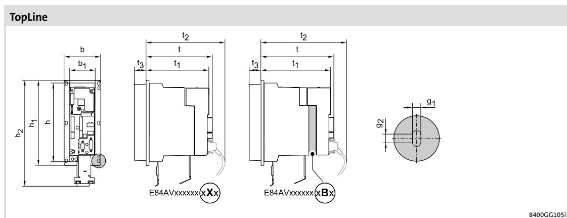
Fig. 5-9 Device dimensions
