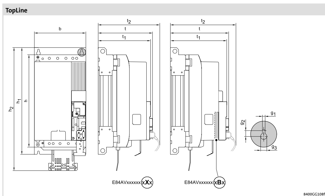
Fig. 5-43 Device dimensions
