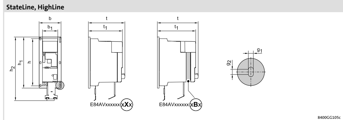
Fig. 5-11 Device dimensions
