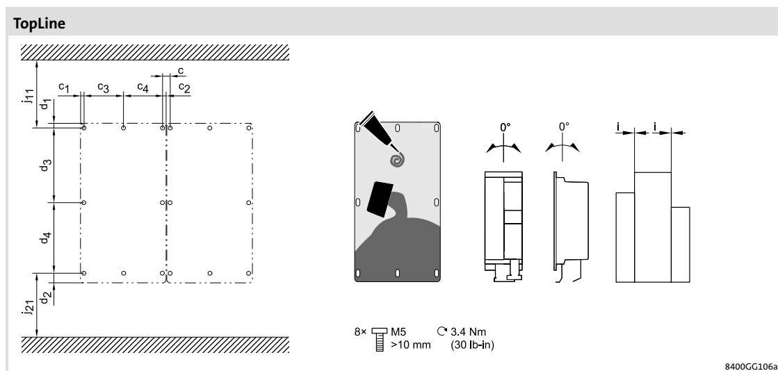
Fig. 5-36 Dimensions for mounting
