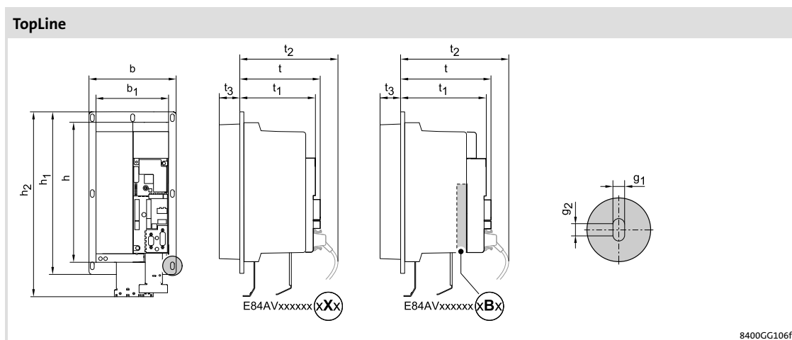
Fig. 5-27 Device dimensions
