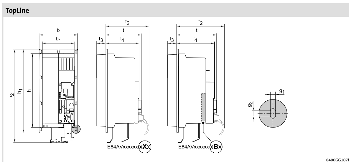
Fig. 5-31 Device dimensions
