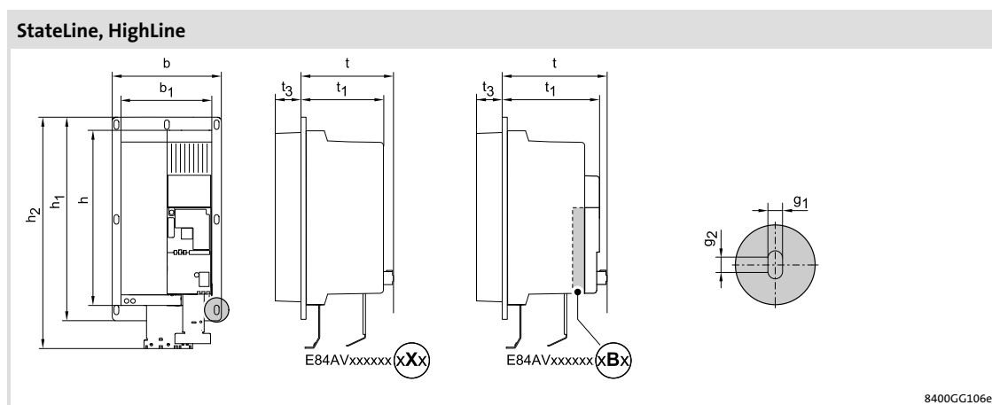
Fig. 5-25 Device dimensions
