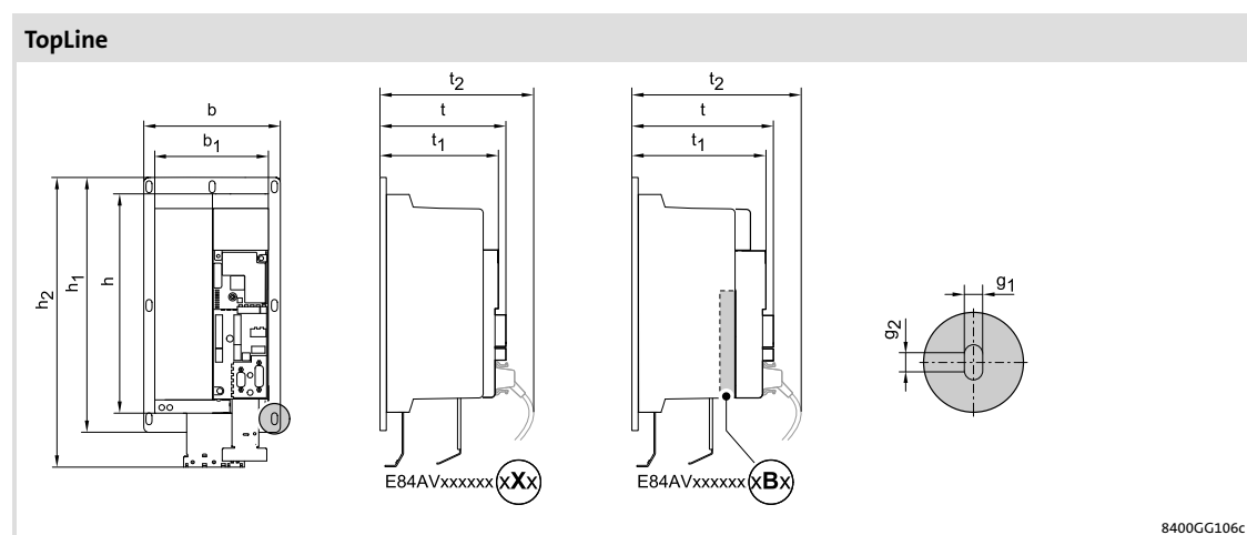
Fig. 5-35 Device dimensions
