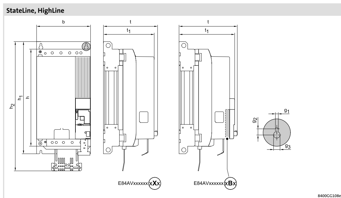
Fig. 5-41 Device dimensions
