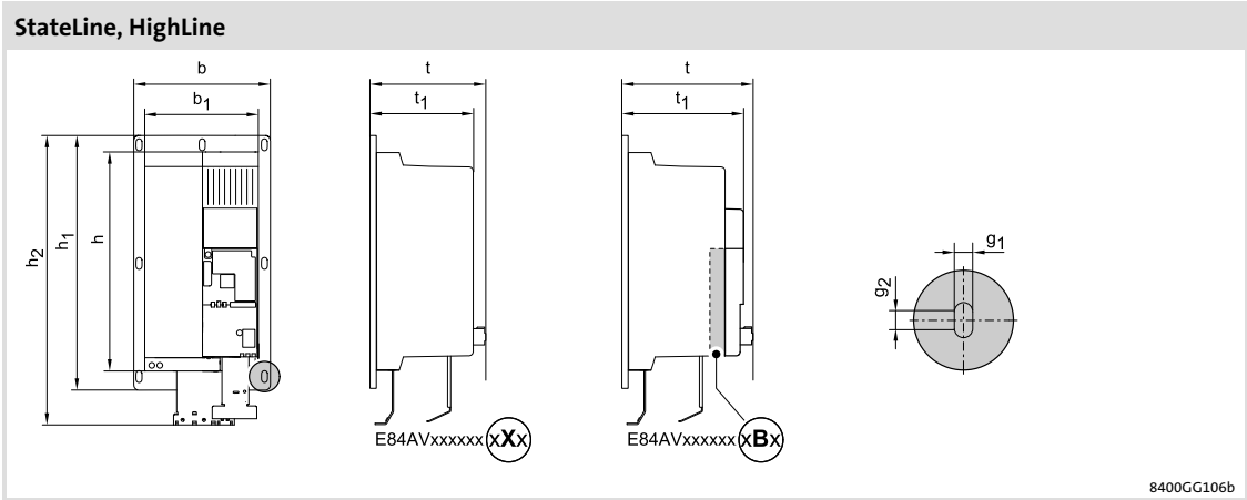
Fig. 5-33 Device dimensions
