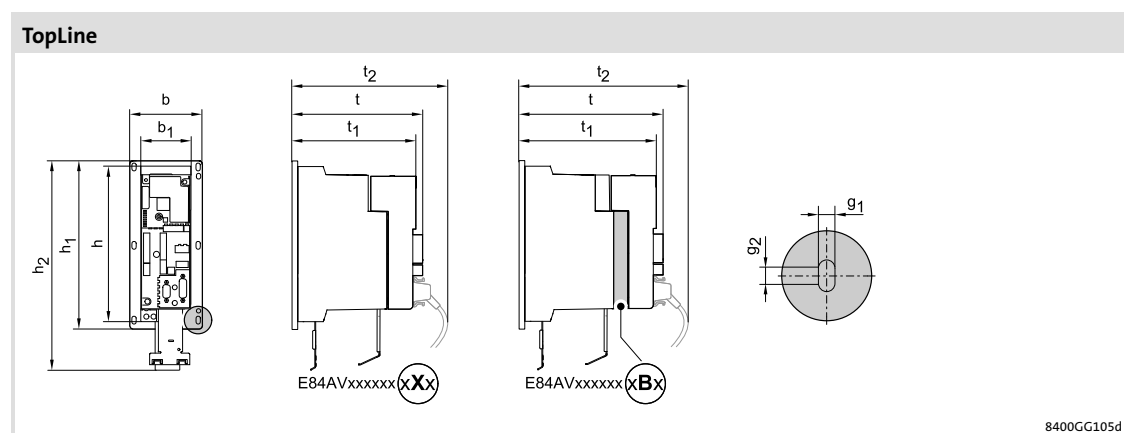
Fig. 5-13 Device dimensions
