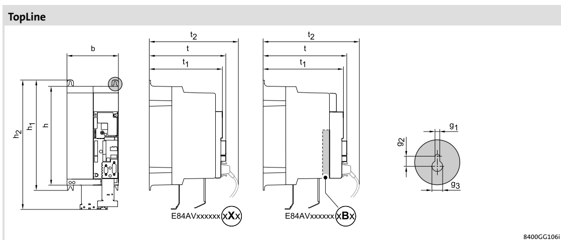
Fig. 5-21 Device dimensions
