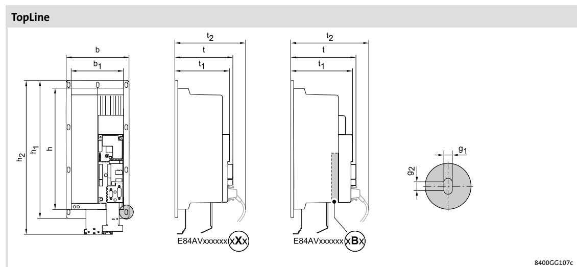
Fig. 5-39 Device dimensions
