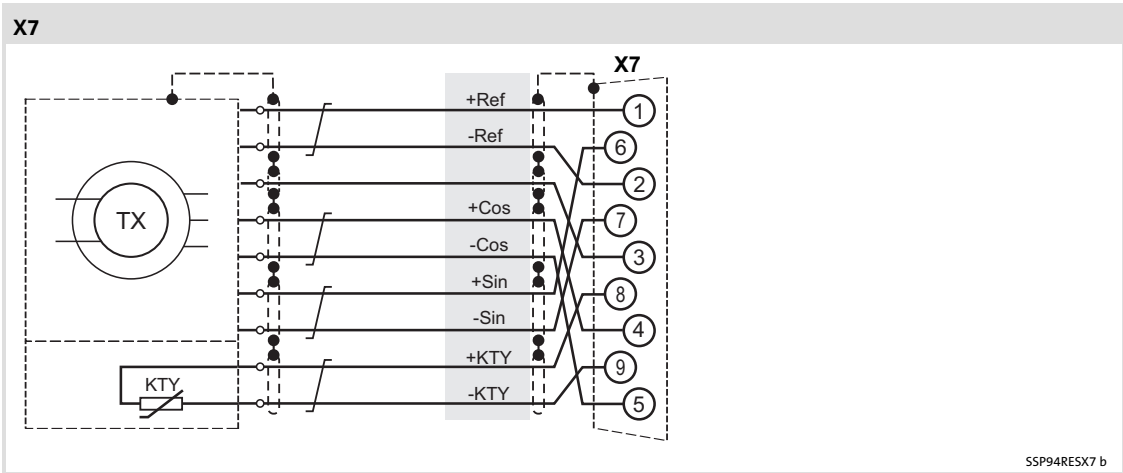
Fig. 6-45 Wiring principle
