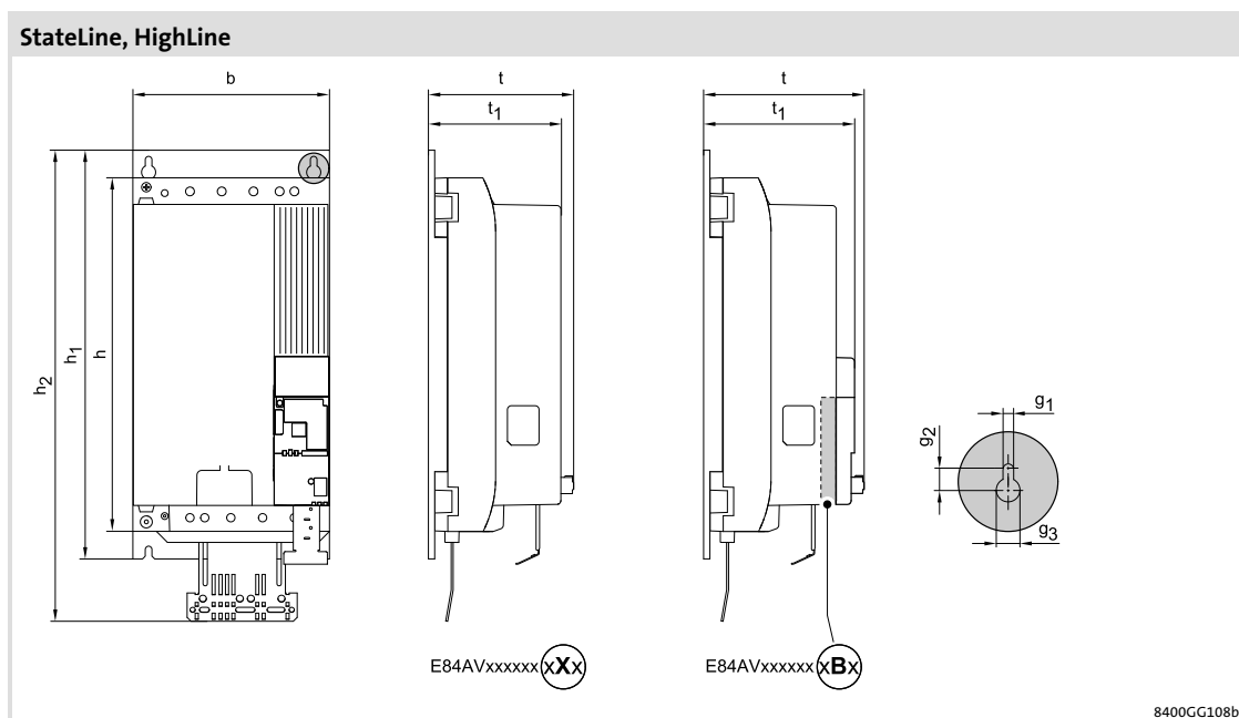
Fig. 5-45 Device dimensions
