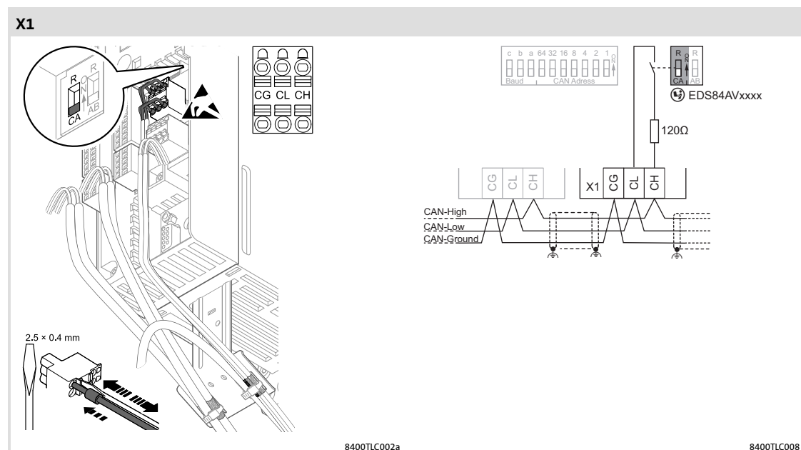
Fig. 6-30 CANopen connection
