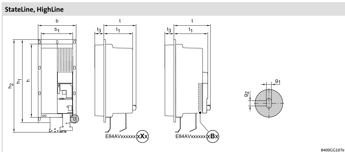
Fig. 5-29 Device dimensions
