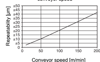
Repeatability as a function of the conveyor speed
