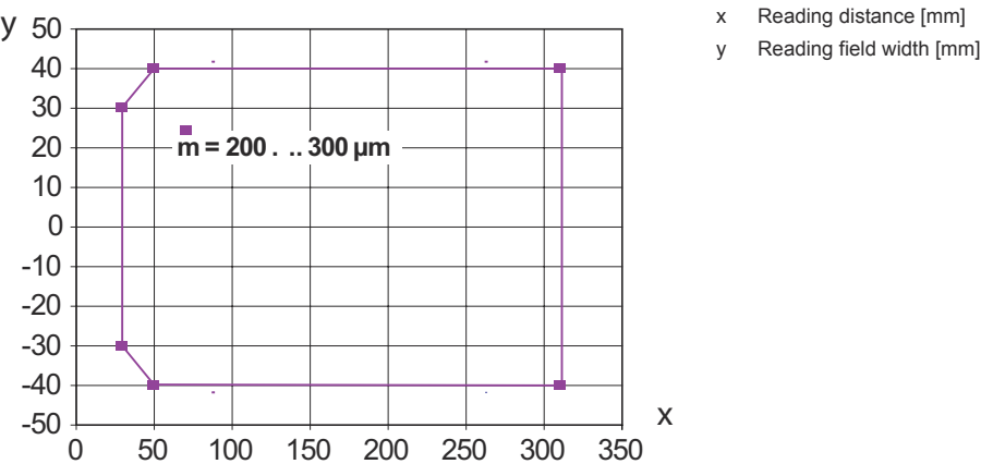
Reading field curve for module m = 0.2 ... 0,3 mm
