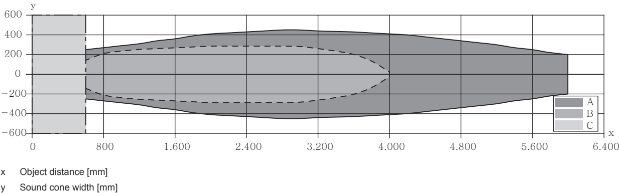
Typ. response behavior
