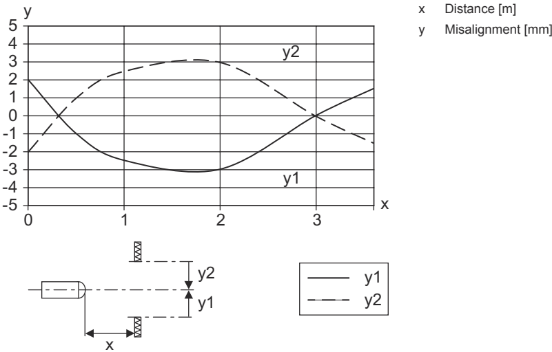
Typ. response behavior (TKS100x100)
