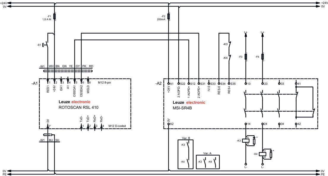
RSL 410 with MSI-SR4B safety relay
