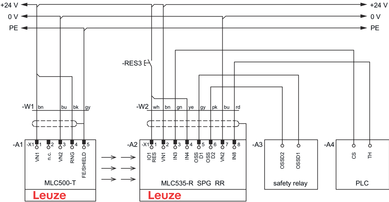
Operating mode 5: circuit diagram example with Smart Process Gating (SPG)
