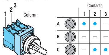
3-position selector switch
