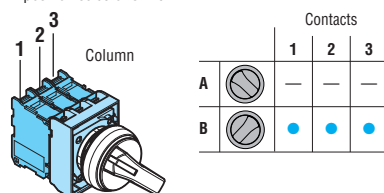
2-position selector switch
