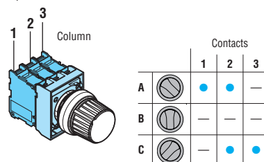
3-position selector switch
