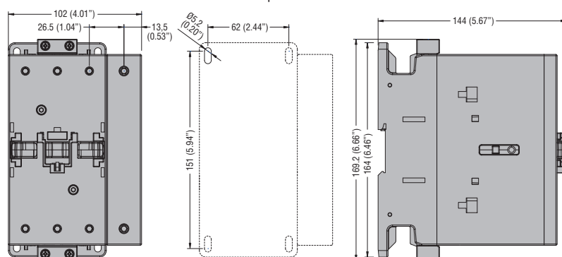
BF95T4A... - BF115T4A... - BF150T4A... four poles
