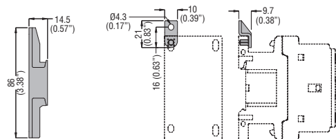
BFX8902 fixing brackets
