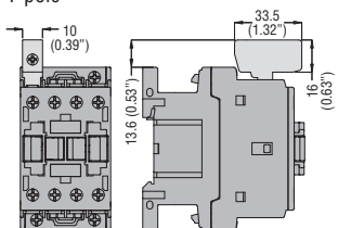
G231 terminal 1-pole
