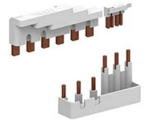
Rigid connecting kits for star-delta starter. For BF40...BF94 (L/Δ) BF26...BF38 (Λ) BFX3332
