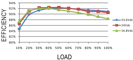
DDR-240B-48
