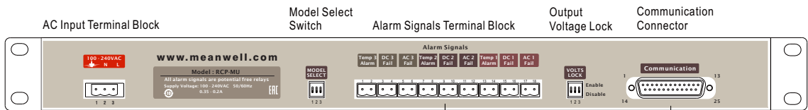
AC Input Terminal Block
