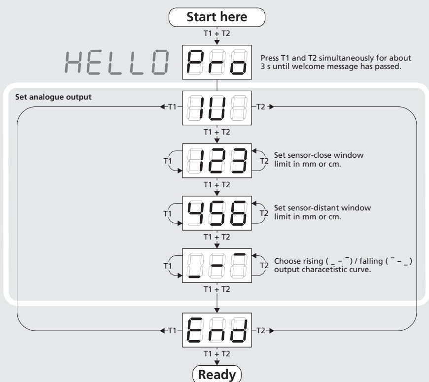
Diagram 1: Set sensor parameters numerically using LED display
