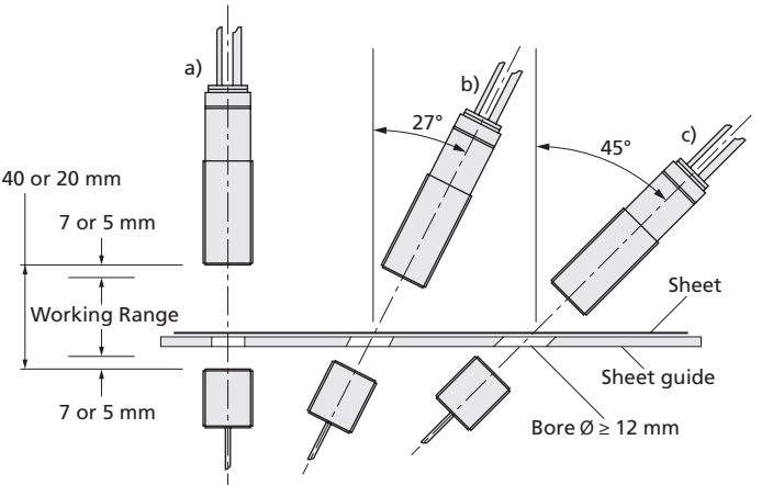
Fig. 3: Mounting and installation positions
